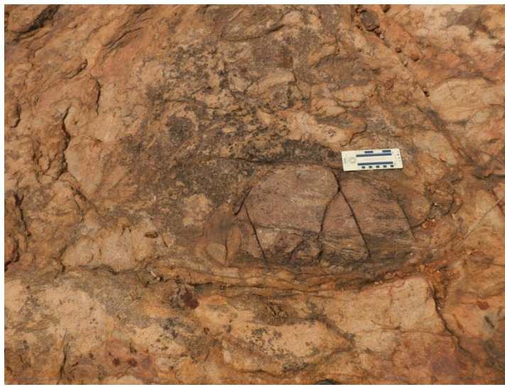
Fig.5 Enclave of Khondalite within felsic gneiss
