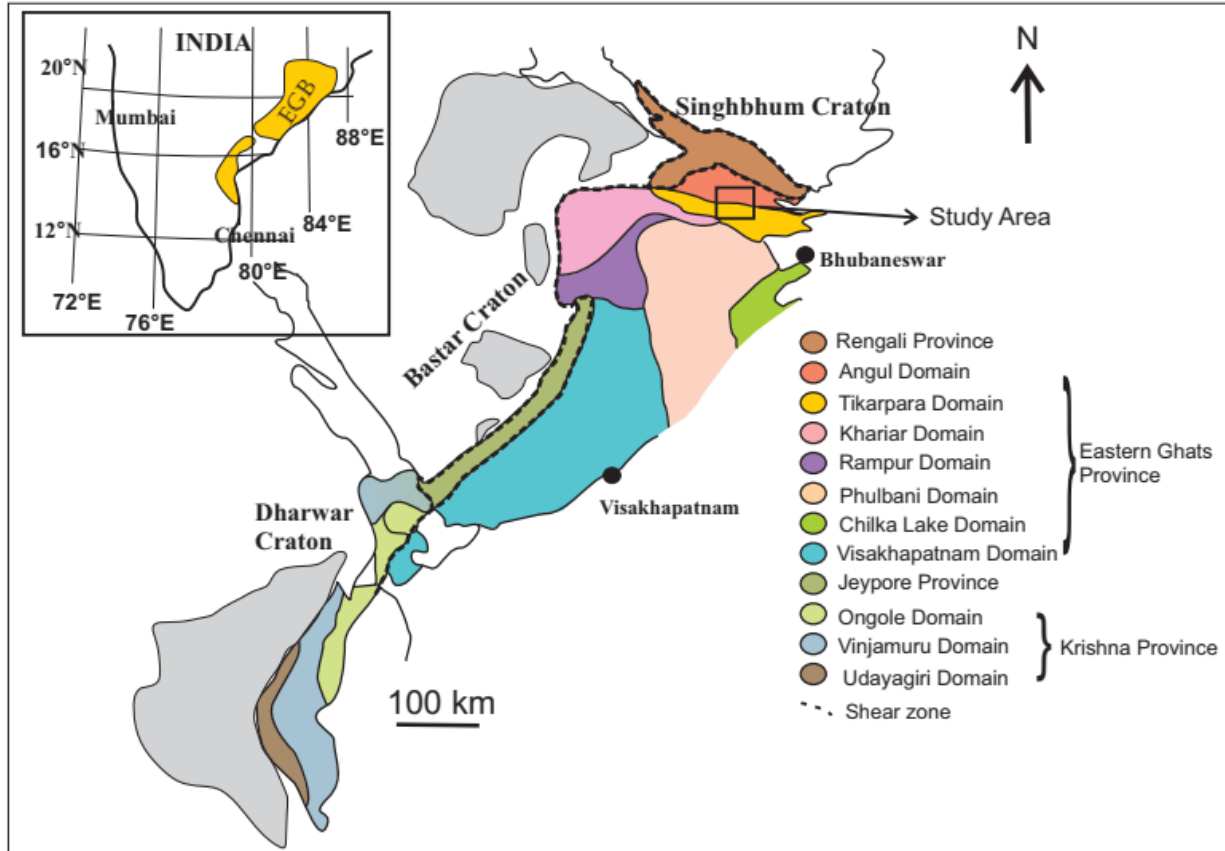
Figure.1 Geological map of the Eastern Ghats Belt (Modified after Dobmeier and Raith, 2003) showing the present study area.
